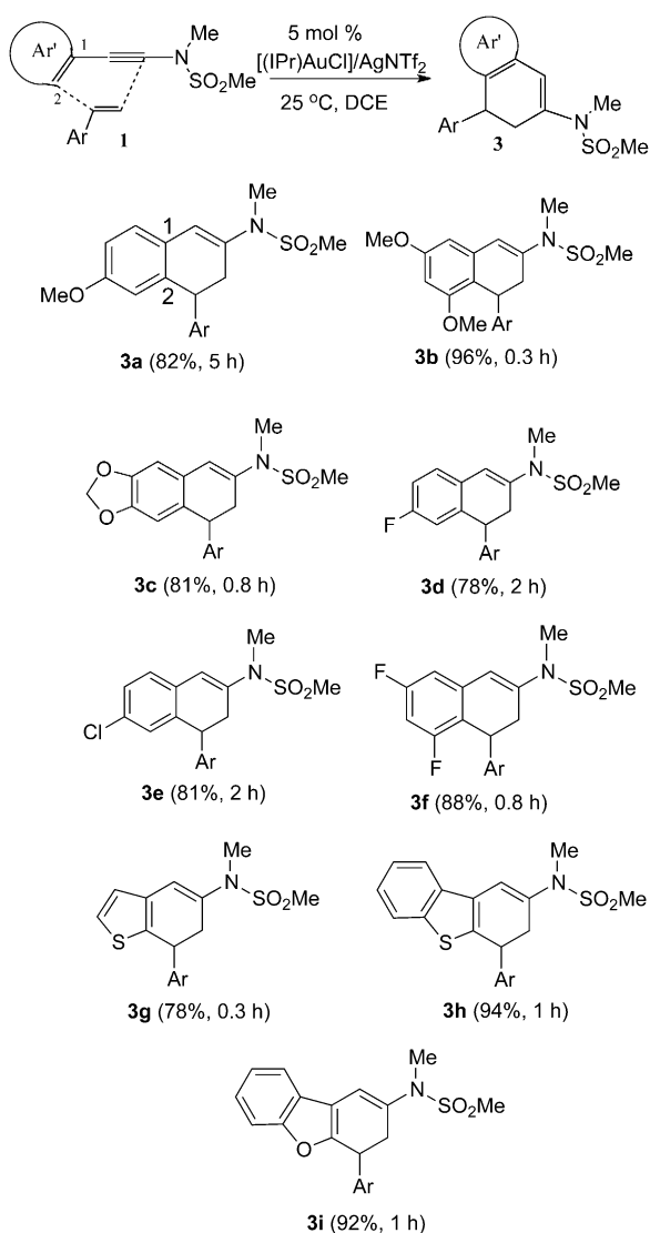
Scheme 3. Cycloadditions of 4-methoxyphenylethene with various aryl-nylamides. Concentration of substrate = 0.1 M, Ar = 4-MeOC 6 H 4 . Reaction times and yields are given in parentheses. Yields are reported after purification.
