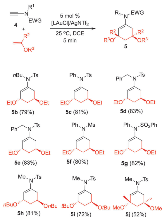
Scheme 4. Scope of gold-catalyzed [2+2+2] cycloaddition. Concentration of 4 = 0.1 M, EWG = electron-withdrawing group, L = P( t Bu) 2 ( o -biphenyl). Yields are given in parentheses and are reported after purification.
